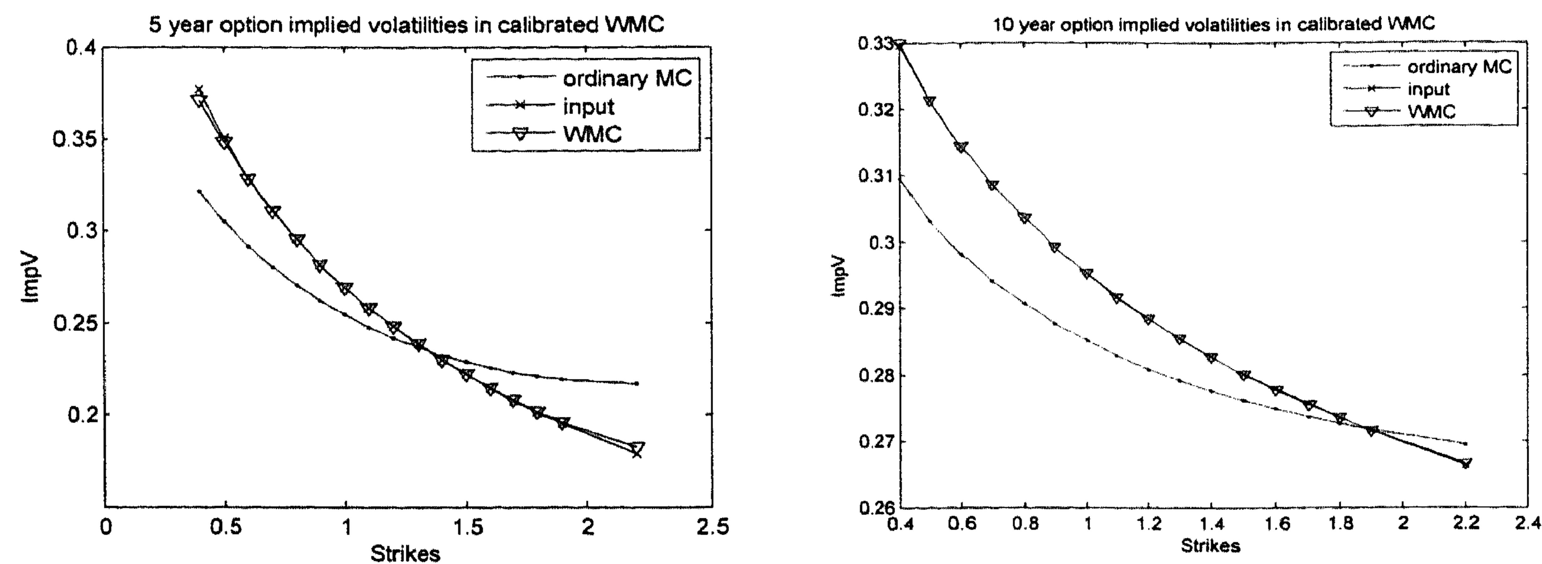
Figure 4.4: The 5 and 10 year option implied volatilities produced by WMC compared against the input market implied volatilities.
