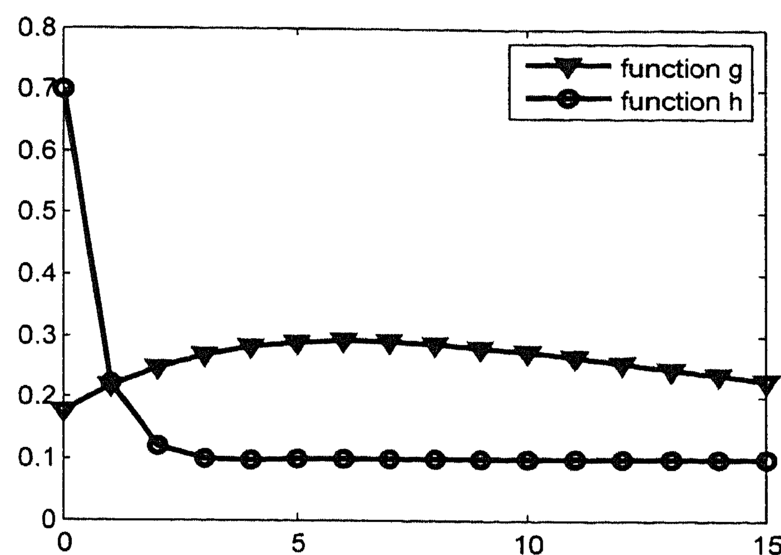
Figure 4.3: The calibrated g(\cdot) and h(\cdot) functions.
