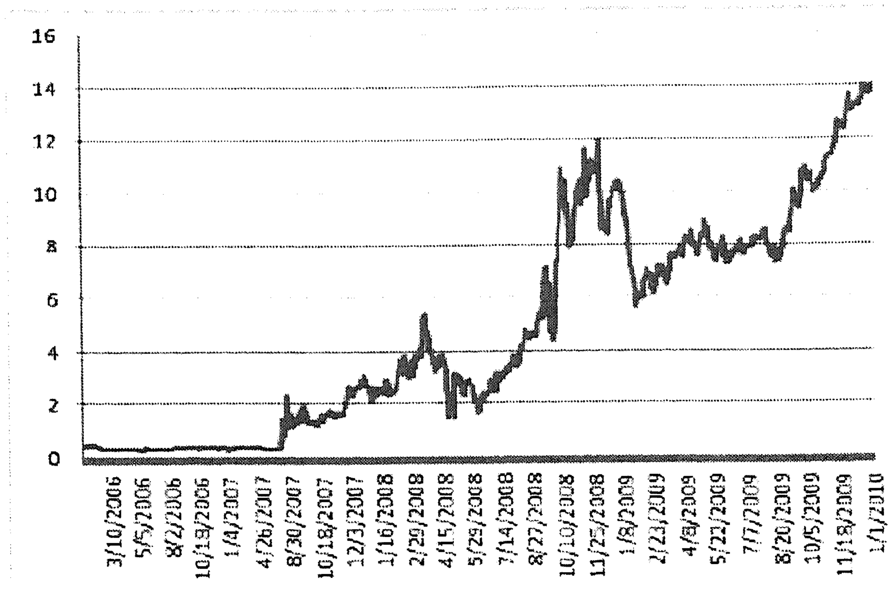
Figure 6.1: Basis spread between 5y 3 month tenor swap rates and 5 year 6 month tenor swap rates, from 02-01-2006 to 02-01-2010, EUR market [78]
