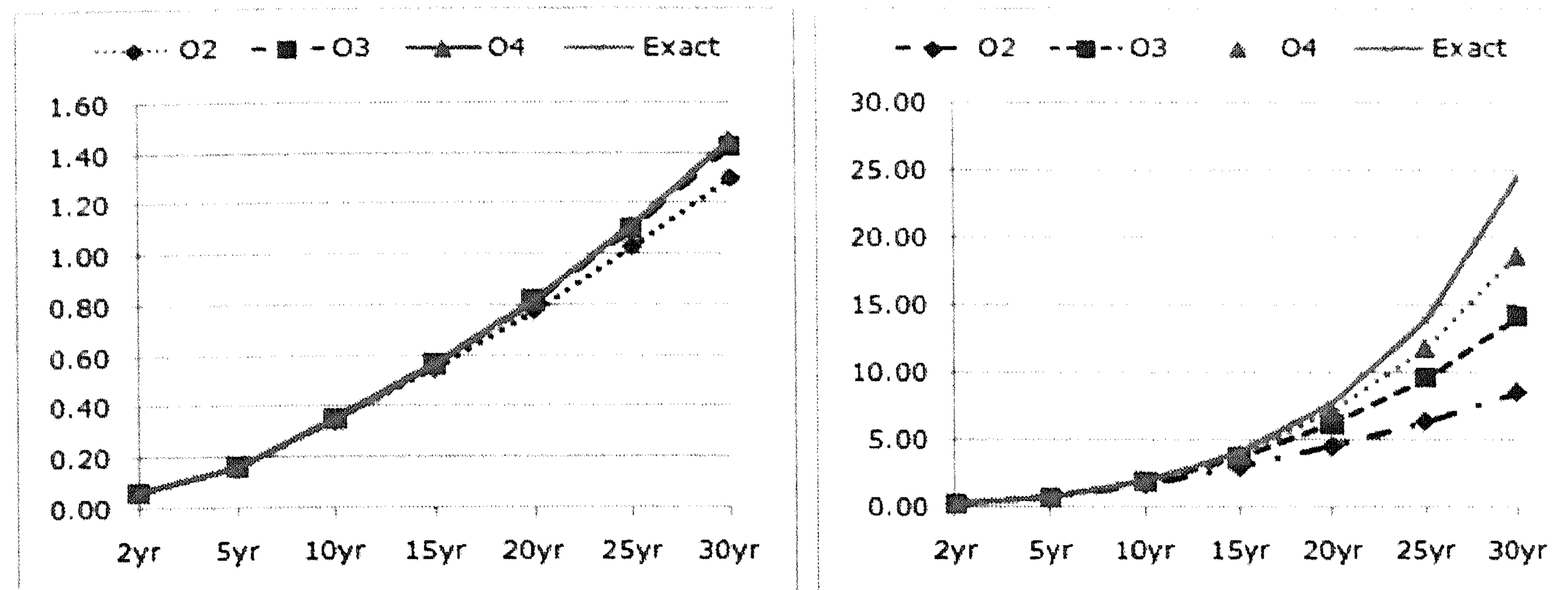
Figure 2.1: Accuracy of the expansion solution (2.4.5) for two-factor log-normal model. Left-hand side: low volatility, i.e. \sigma_x = 20\% and \sigma_y = 45\% ; Right-hand side: high volatility with \sigma_x = 40\% and \sigma_y = 45\% .
