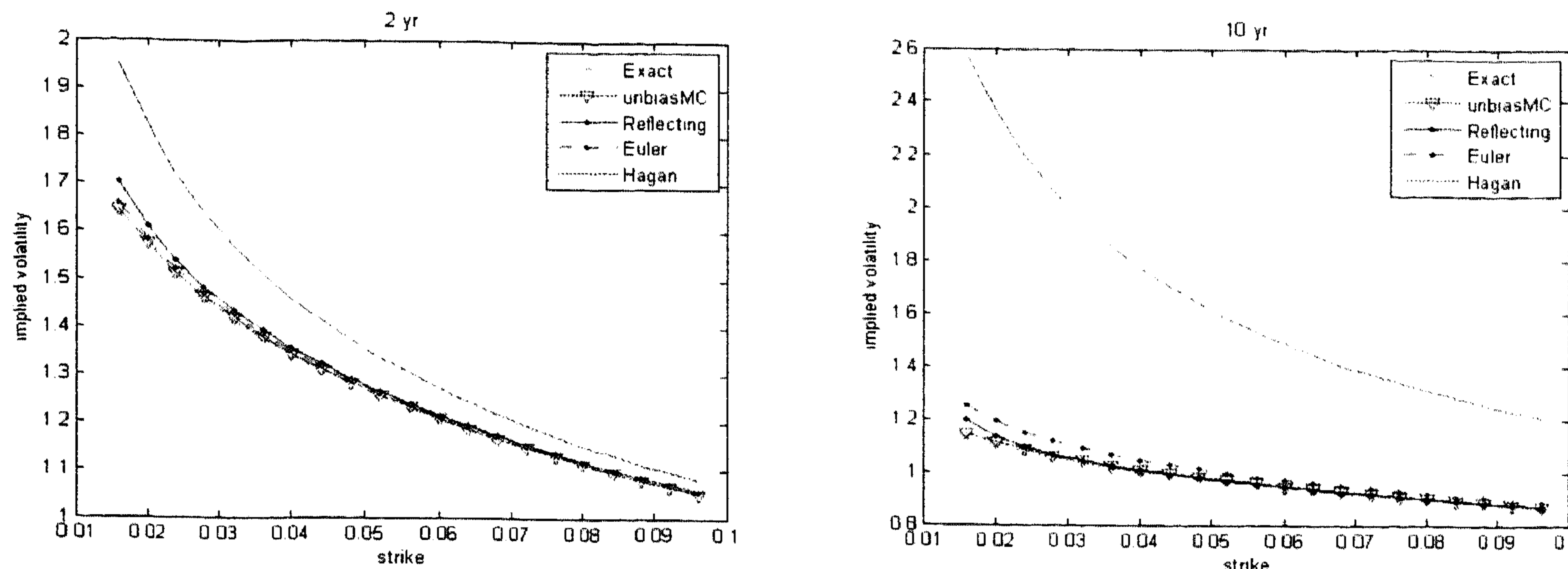
Figure 3.6: Comparison for the CEV process of the implied volatilities generated by different methods; Maturities are 2 and 10 years, and parameters \alpha = 0.0 , S(0) = 0.04 , \sigma(0) = 0.2 and \beta = 0.4 .
