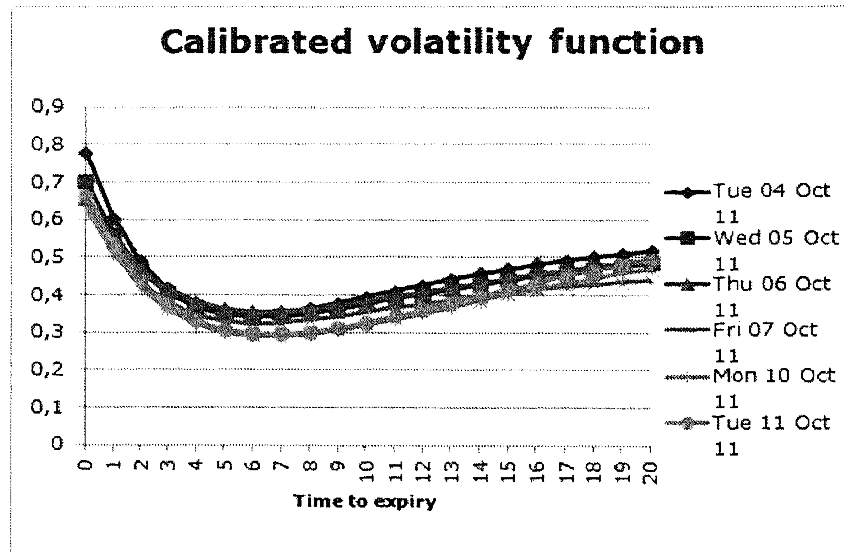
Figure 5.10: The plot of calibrated time-homogeneous volatility functions across several spot dates.
