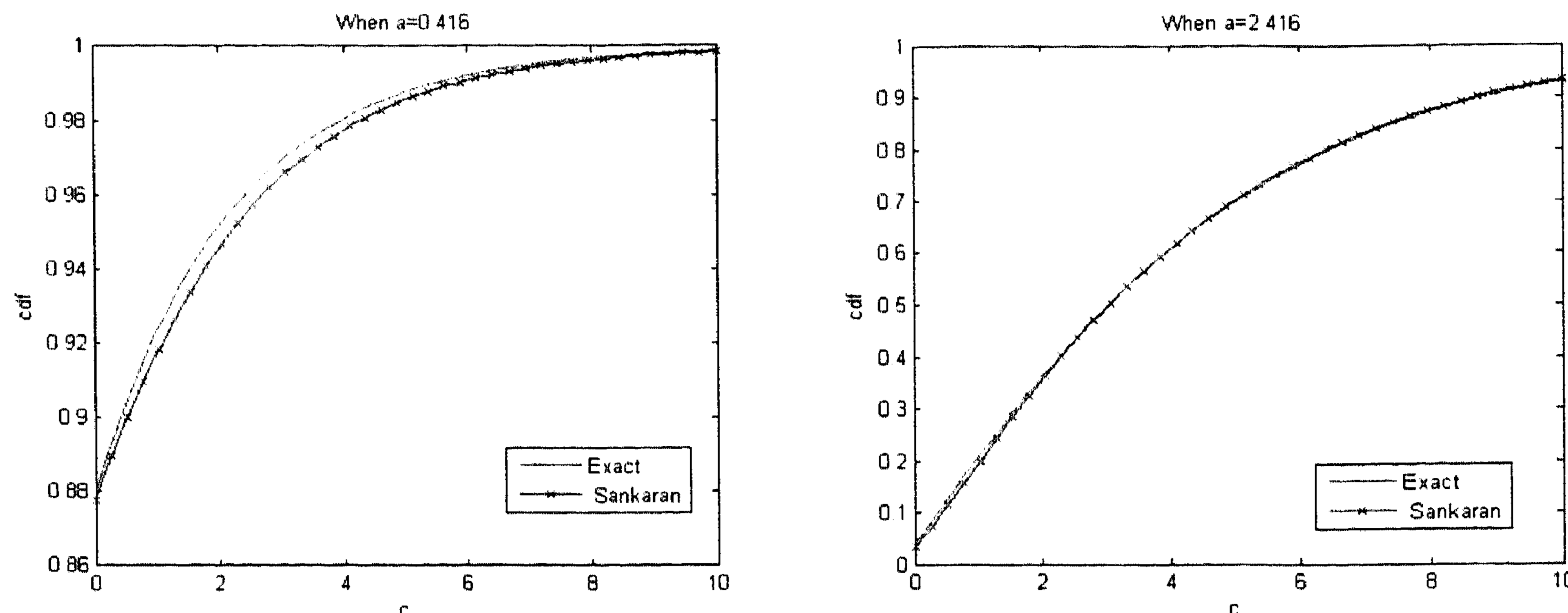
Figure 3.2: Comparison of the quality of Sankaran's approximation for two sets of parameters. Degree of freedom parameter b is set to 0.423 for both cases, but parameter a is lower in the left-side plot, a = 0.416 than in the right-side plot, a = 2.416 .
