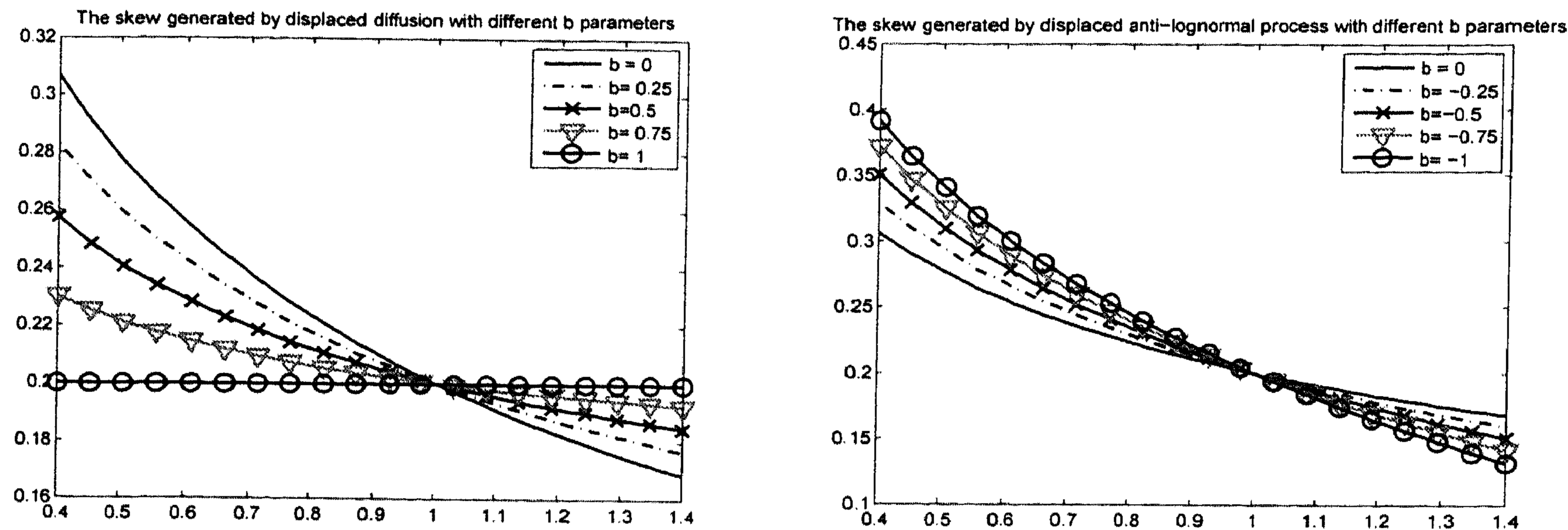
Figure 5.14: LHS: The steepness in skews given parameters b in Eq. (5.5.2). RHS: The steepness in skews given parameters b in Eq. (5.5.2).
