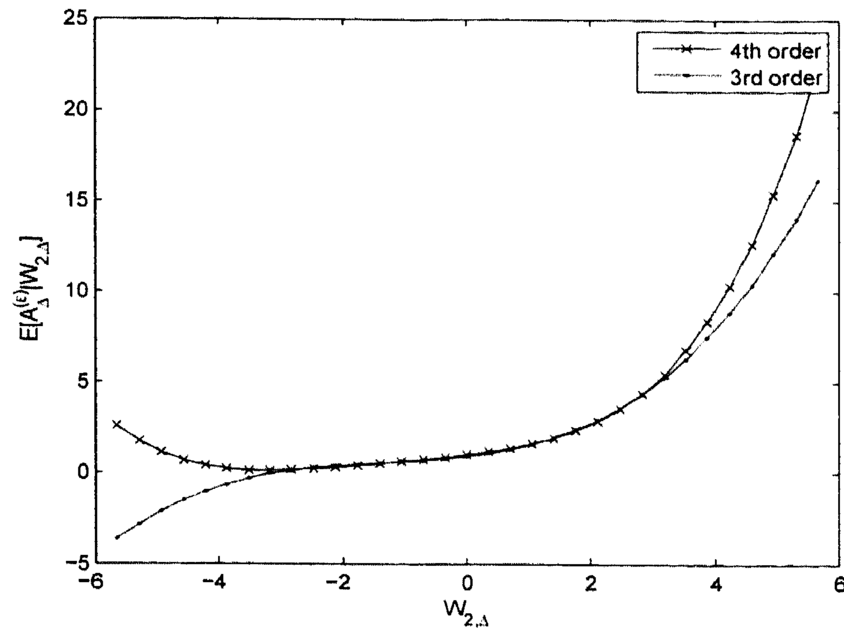
Figure 3.3: Illustration of formula (3.3.15) for the conditional mean \mathbb{E}[A(\Delta)|W_2(\Delta)] ; including the first three expansion terms versus the first four terms.
