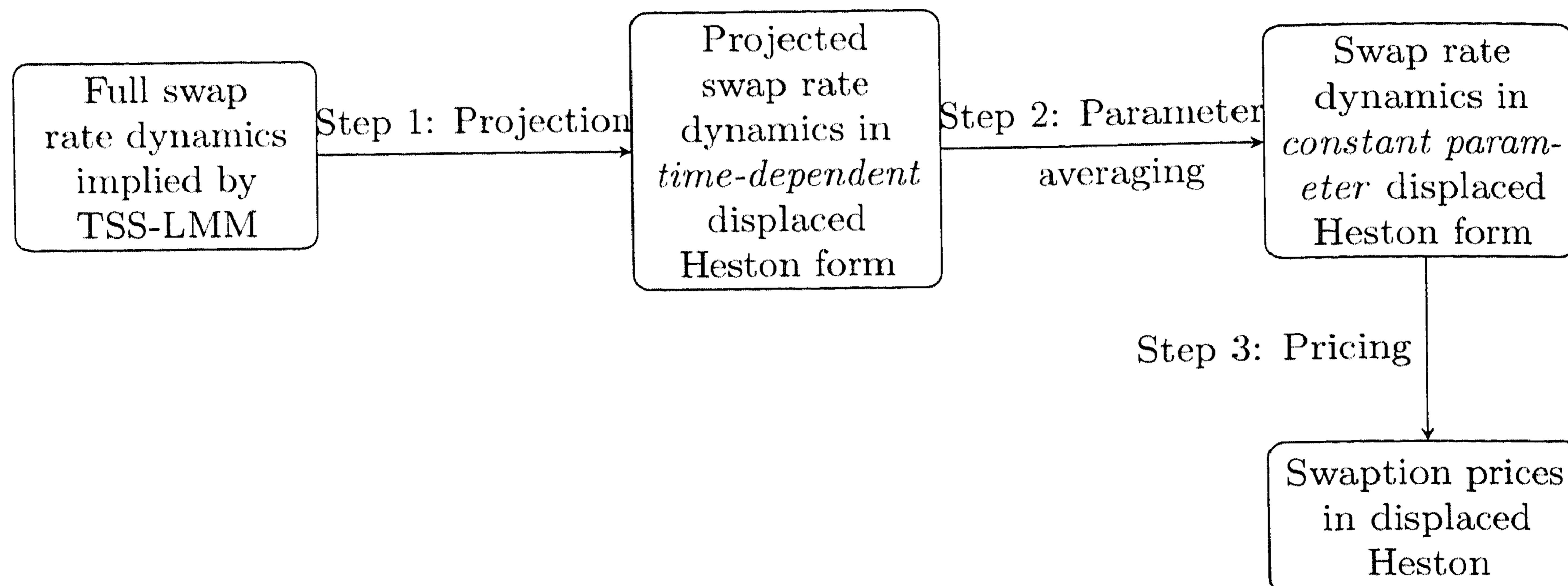
Figure 5.2: Model mapping procedure for the TSS-LMM
