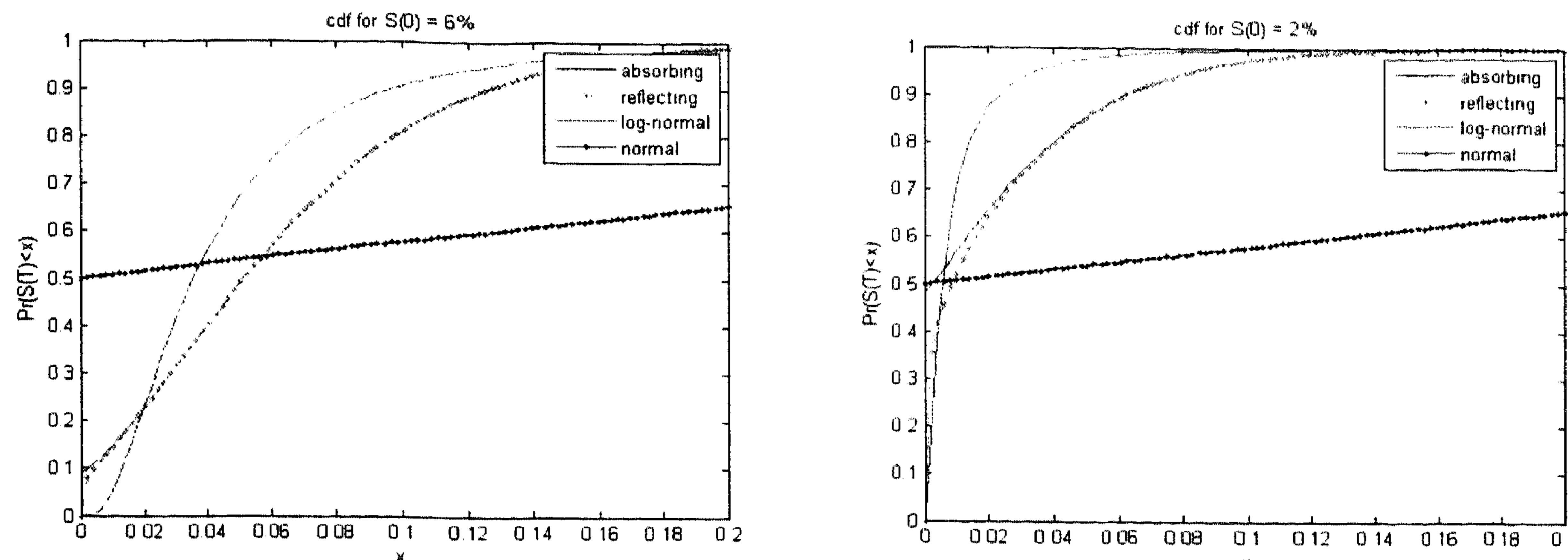
Figure 3.1: Comparison of the exact cumulative distribution of the CEV process versus the log-normal and normal distributions at T = 0.25 for S(\Delta) given different levels of S(0) .
