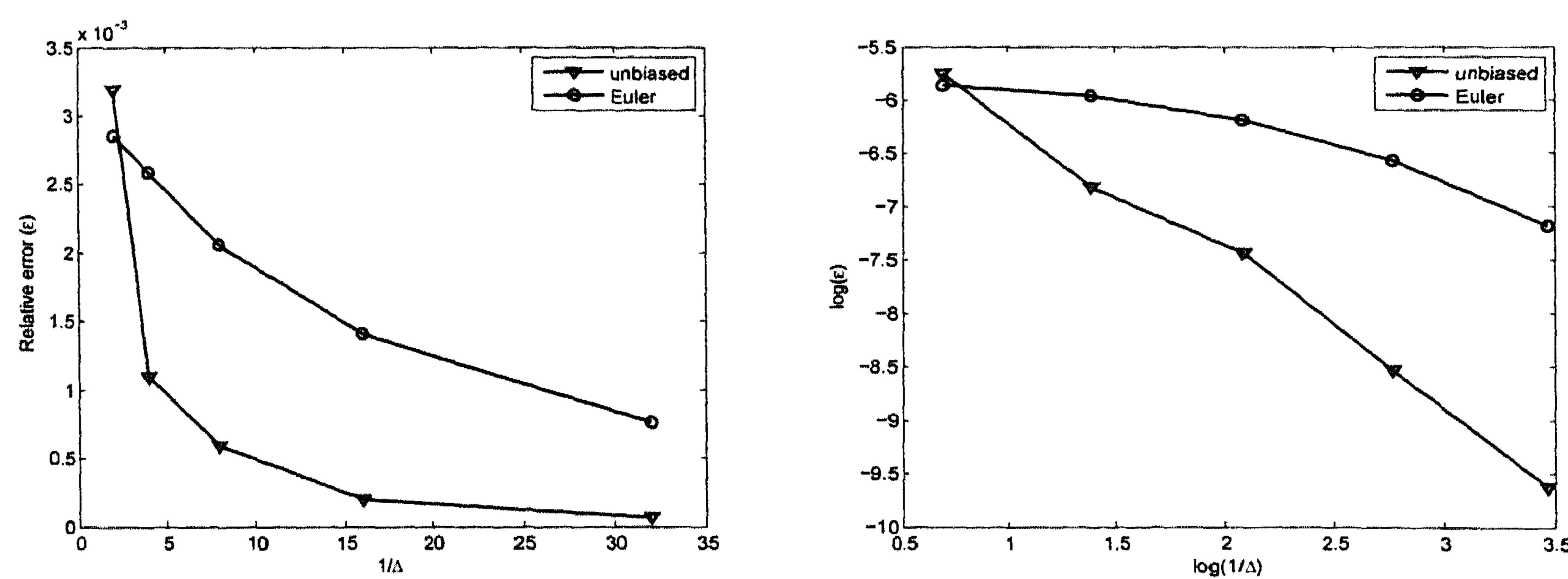
Figure 3.9: Convergence of relative errors, T = 5 ; Test Case IV; error versus time step size, right: same picture in log-log scale.
