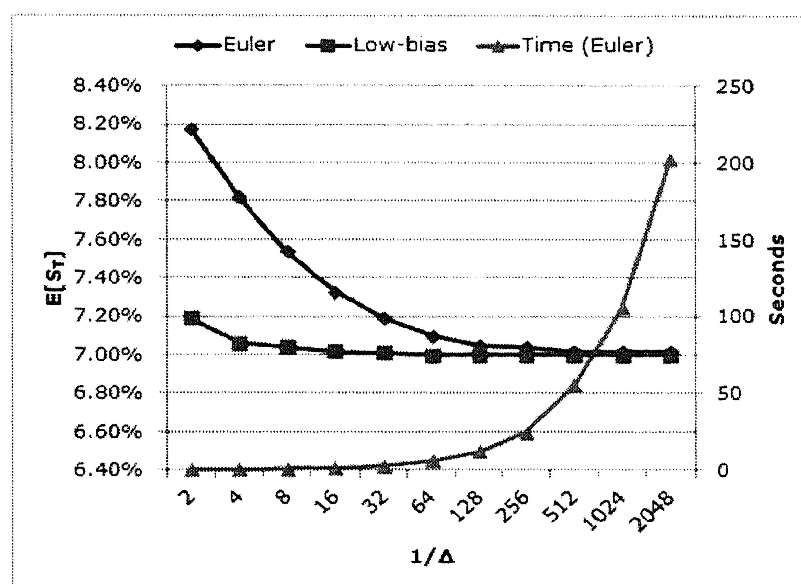
Figure 3.11: Comparison of martingale bias of the low-bias scheme and the truncated Euler scheme for a simulation up to one year in Test Case IV. The computational time of the truncated Euler scheme is plotted against the number of time steps in the secondary y -axis.
