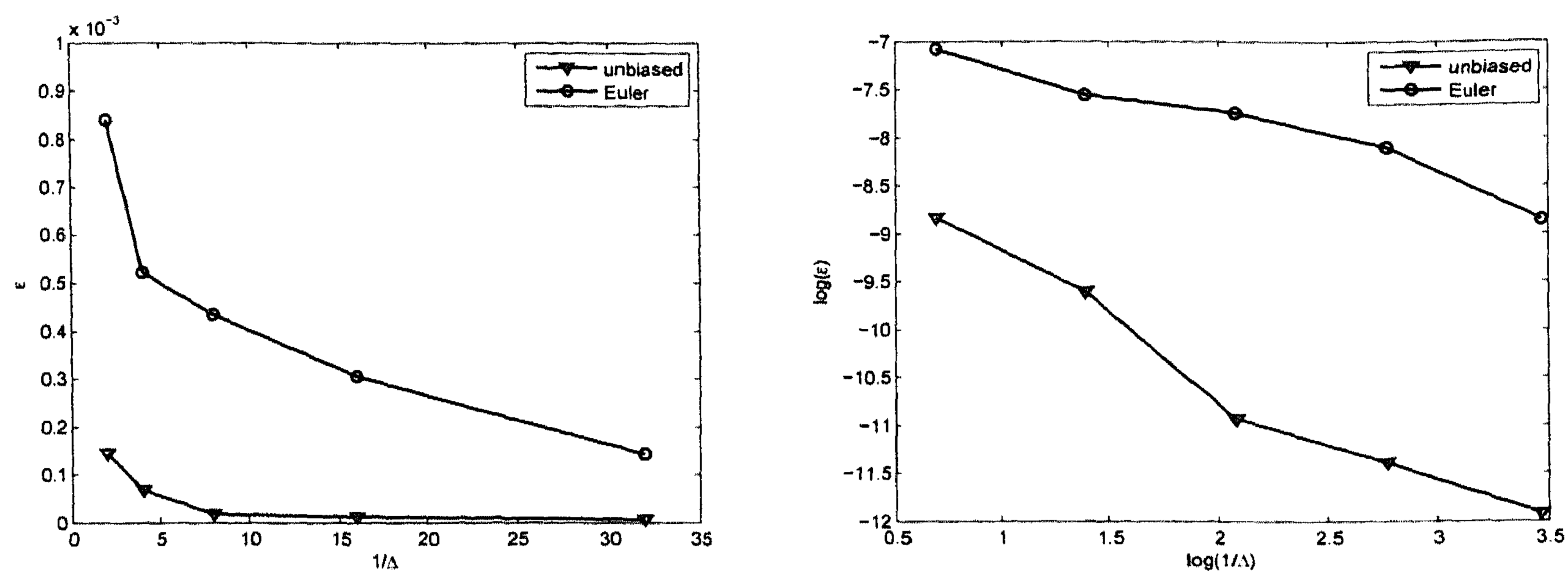
Figure 3.8: Convergence of relative errors; Test Case III; left: error versus time step size, right: same picture in log-log scale.
