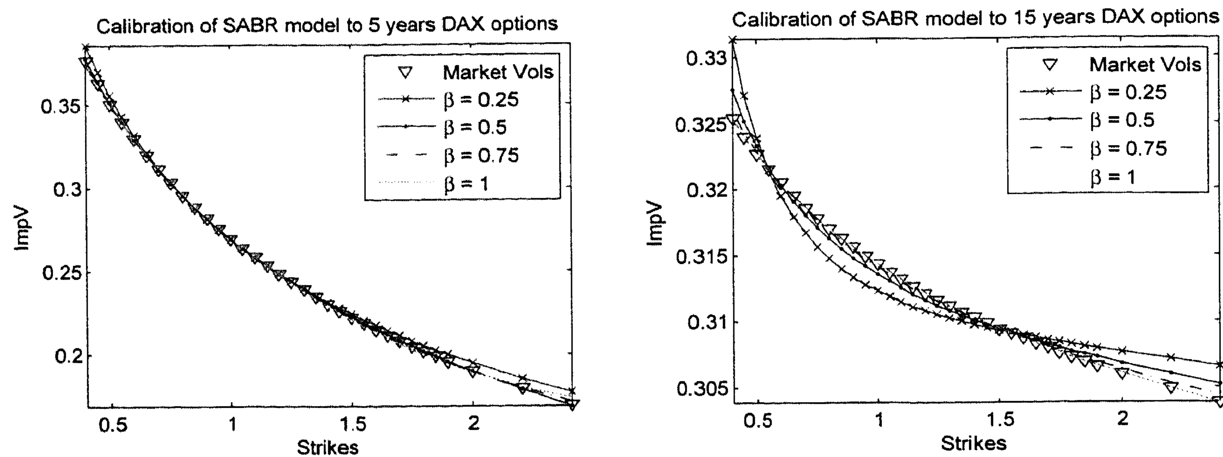
Figure 4.2: Calibration results for the SABR model with different a priori chosen \beta parameters to the implied volatilities of 5 and 15 years maturity.
