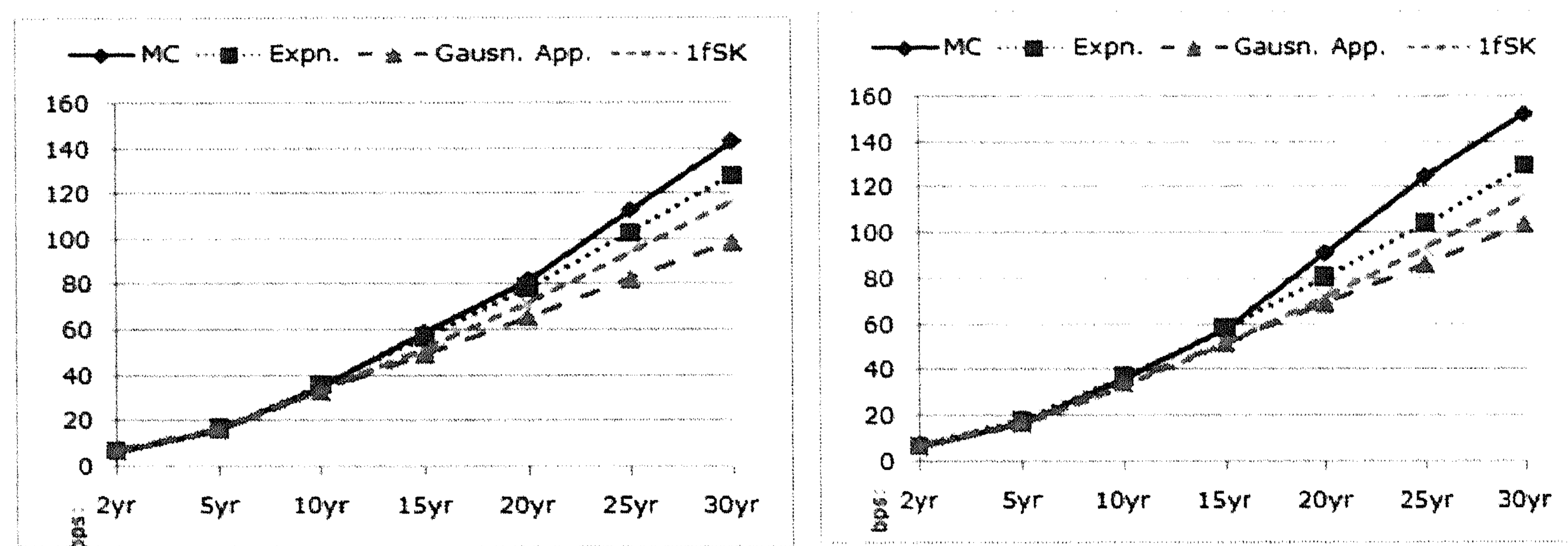
Figure 2.2: Comparison of several convexity correction methods with \beta_x = \beta_y = 1 and two different swap-LIBOR correlations. Left-hand side: the convexity correction in time for \rho_{xy} > 0 . Right-hand side: convexity correction for \rho_{xy} < 0 .
