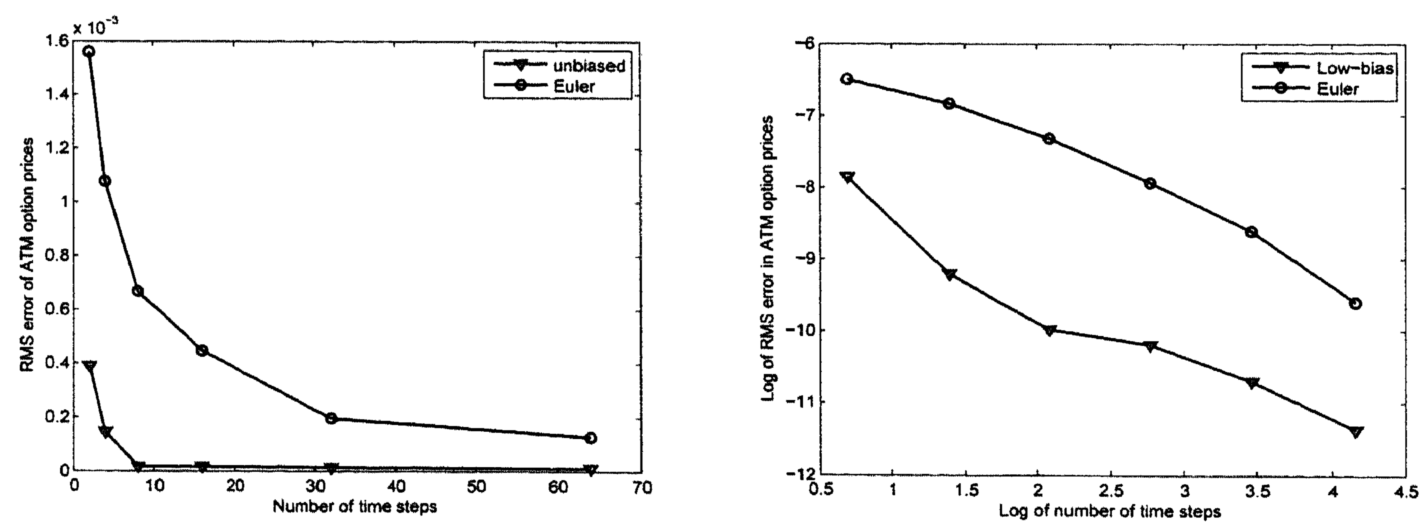
Figure 3.7: Test Case II; Convergence of the estimated RMS error for call options with decreasing time step \Delta .
