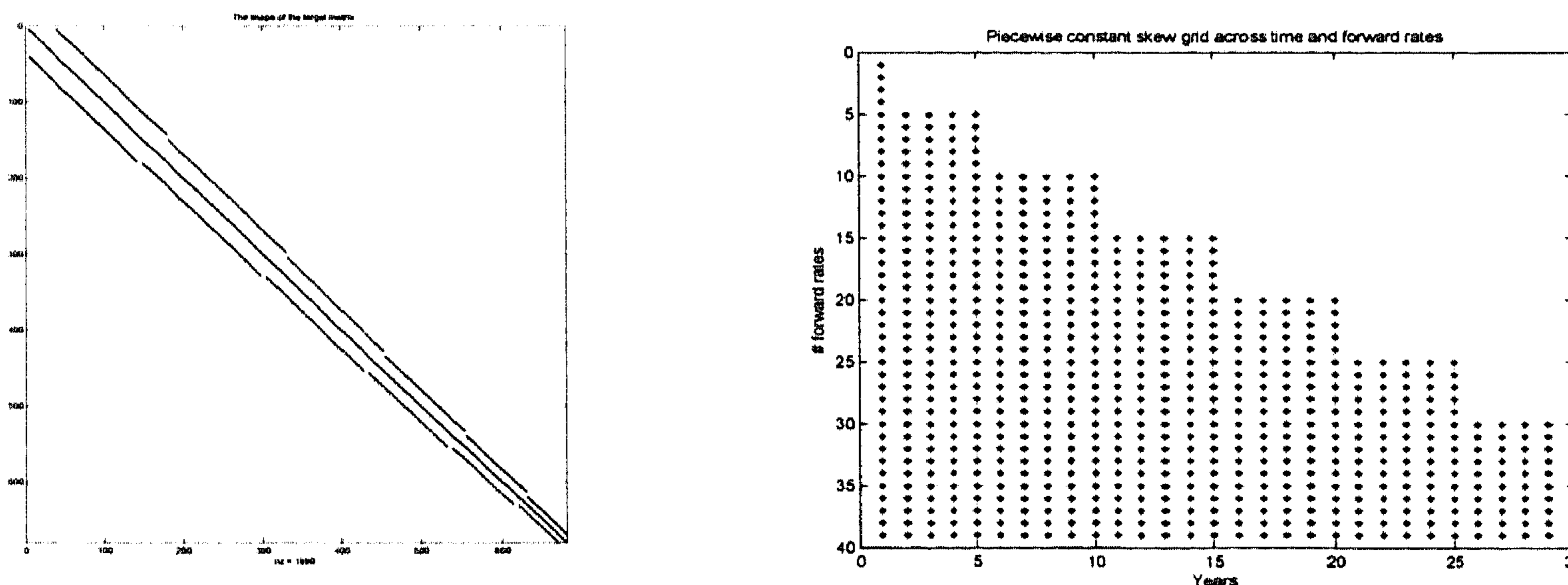
Figure 5.11: LHS: The target matrix M for a 30 by 30 swaption matrix with the time-homogeneity constraint. RHS: A 'skew pattern' for a (30 \times 30) swaption matrix with expiry dates at 1, 5, 10, 15, 20, 25, 30 years.
