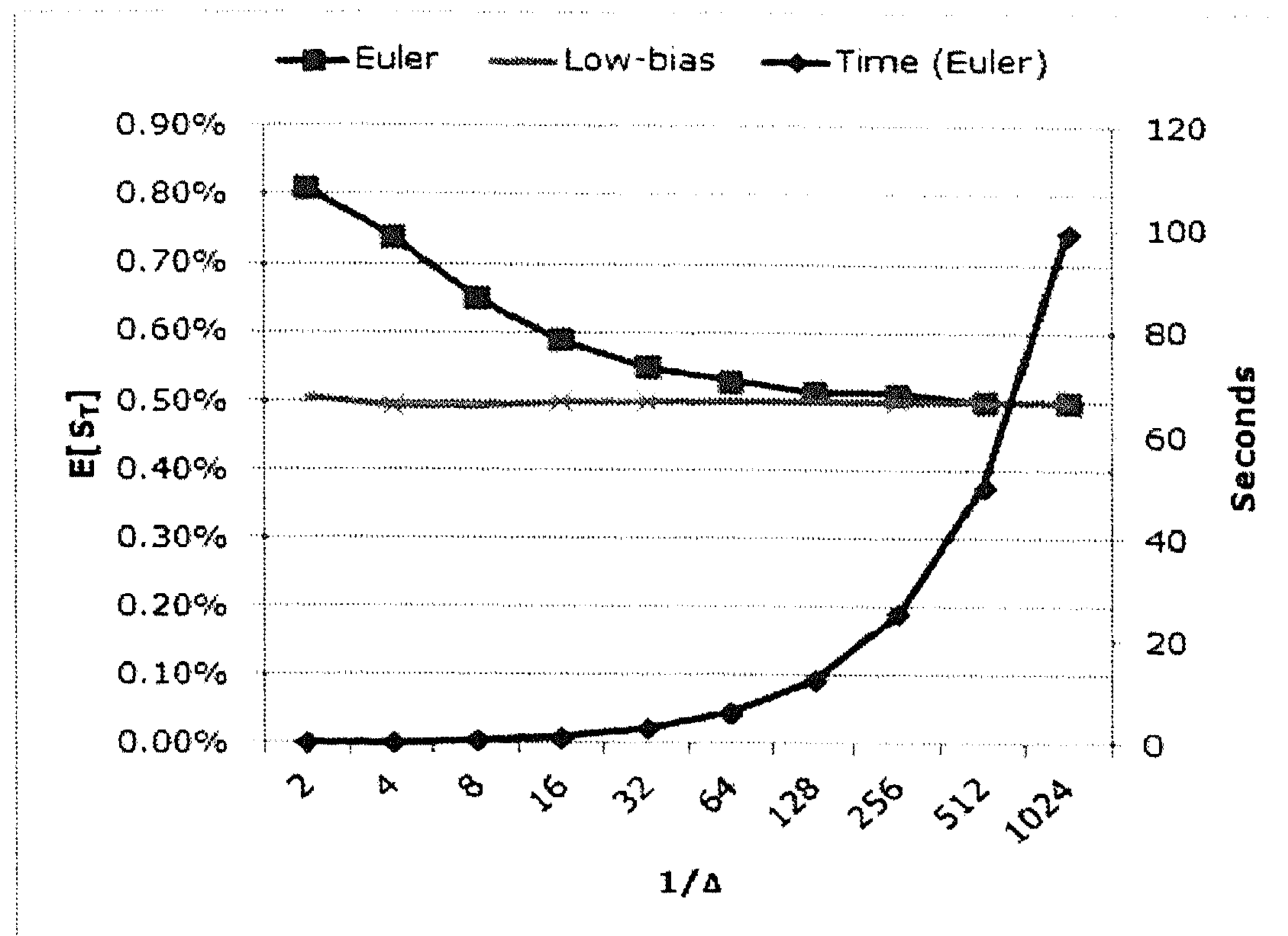
Figure 3.10: Comparison of martingale biases of the low-bias scheme and the truncated Euler scheme for a simulation up to one year in Test Case III. The E[\hat{S}(T)] curves are the discrete approximations of \frac{1}{N} \sum_{i=1}^N \hat{S}(T) , with \hat{S}(T) generated by different discretization schemes. The computational time of the truncated Euler scheme is plotted against the number of time steps in the secondary y -axis.
