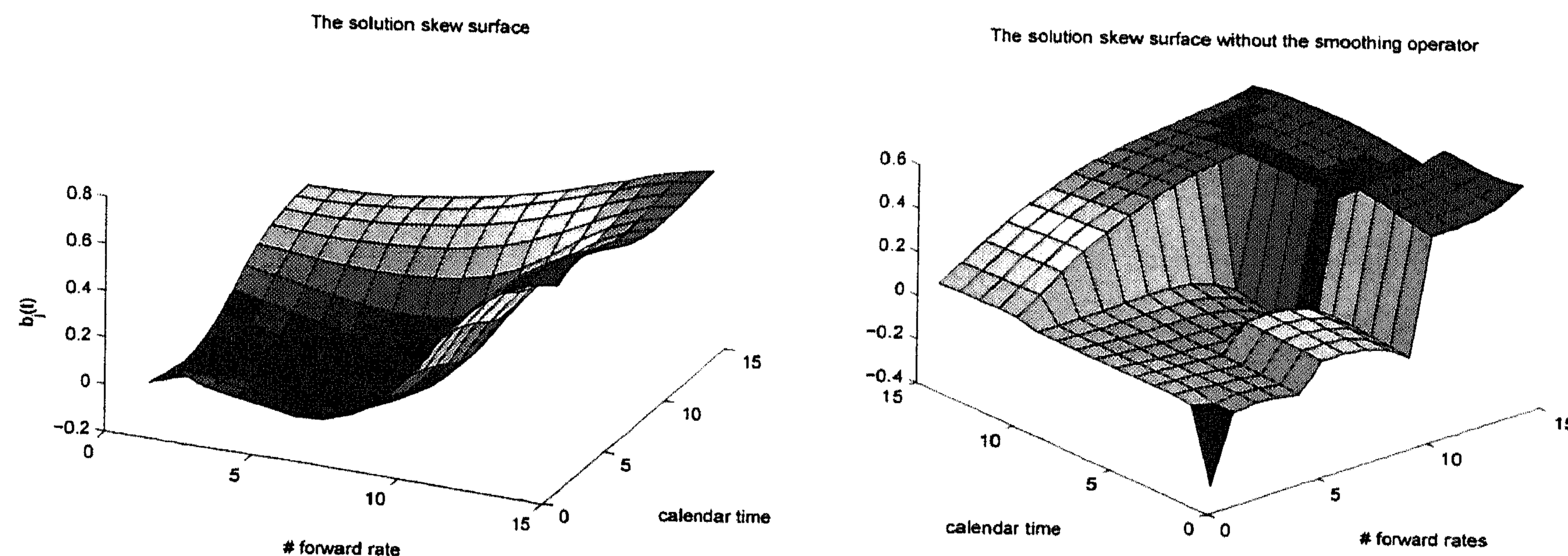
Figure 5.13: The calibrated instantaneous skew surface for the current market data set.
