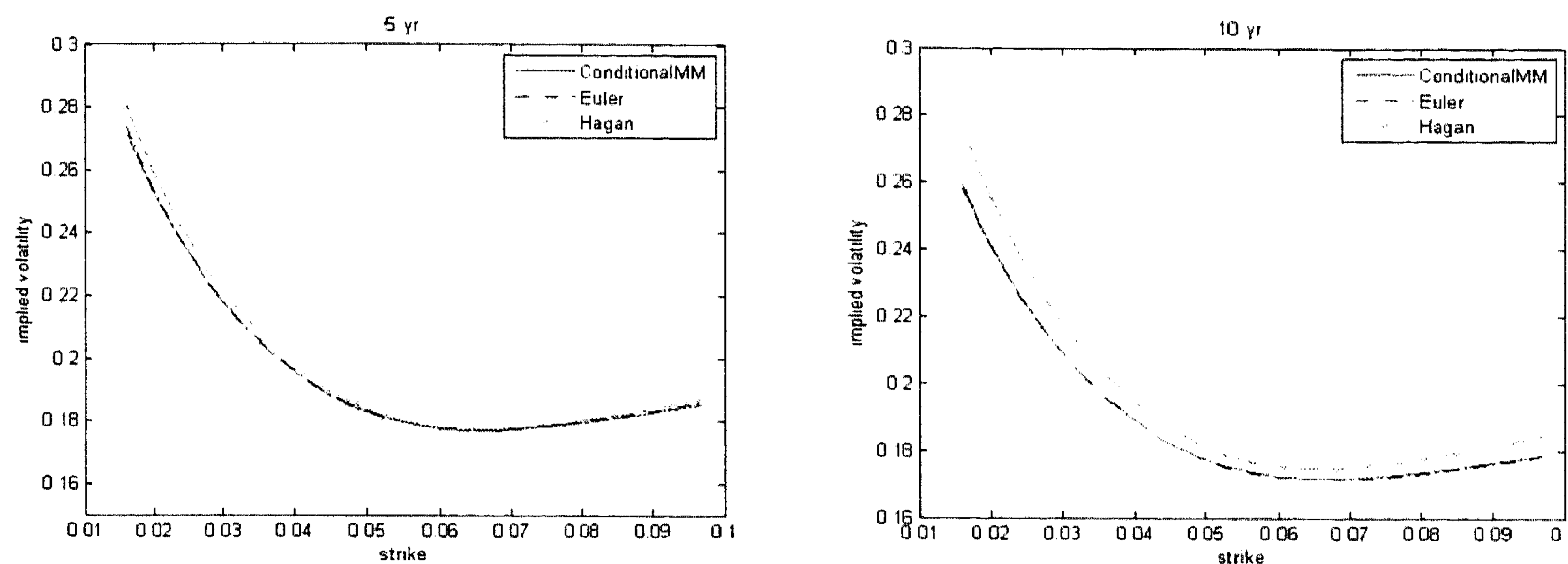
Figure 3.5: Result of the conditional moment-matching log-normal sampling scheme for the integrated variance, simulating 5 and 10 year call option prices under a double log-normal model. A comparison is made with the truncated Euler Monte Carlo scheme, and Hagan’s asymptotic SABR formula. Parameters used are \alpha = 0.3 , \rho = -0.5 , S(0) = 0.04 , \sigma(0) = 0.2 .
