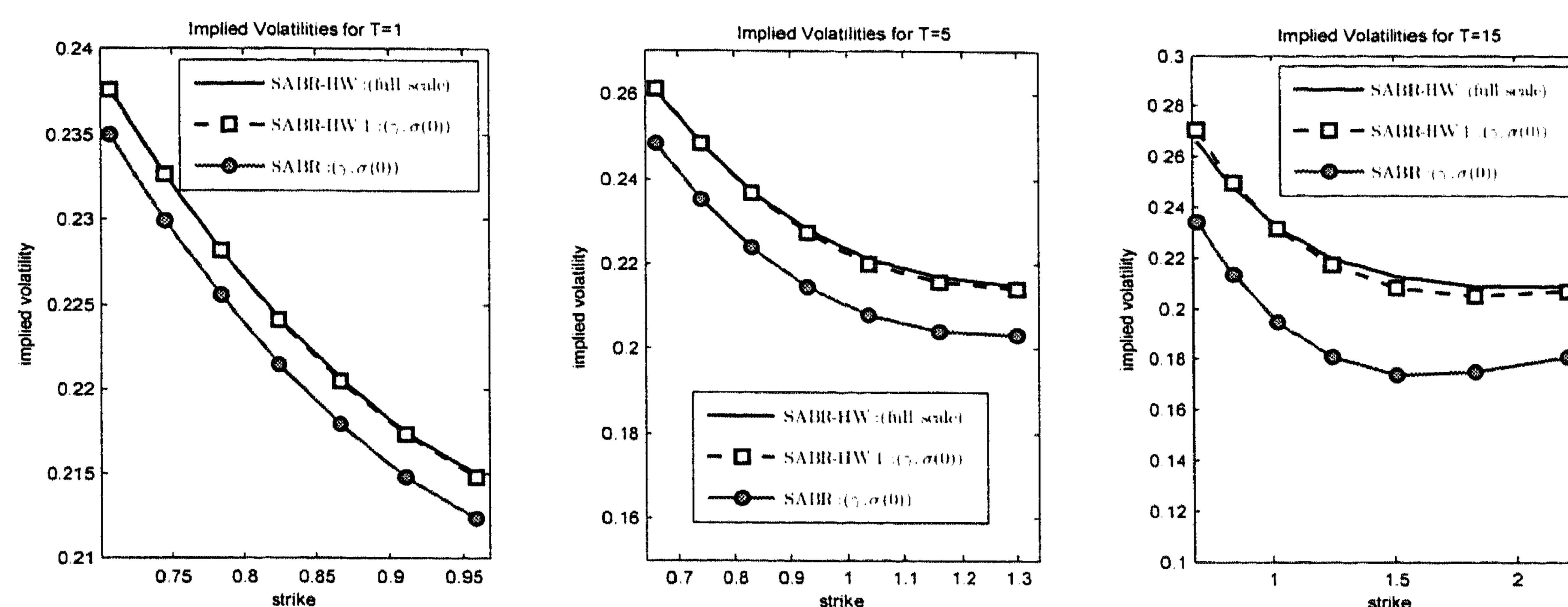
Figure 4.1: Comparison of implied Black-Scholes volatilities for European equity options and parameter set 2 in Table 4.1; For the SABR-HW model, Euler Monte Carlo was used with 100.000 paths and 20T intermediate steps.
