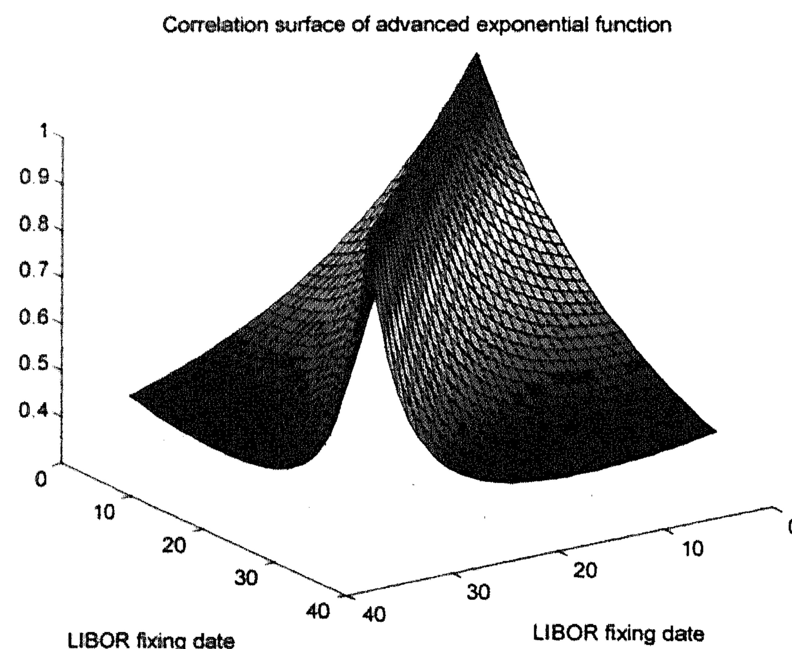
Figure 5.5: Plot of the correlation surface generated by the modified exponential correlation function (5.4.3).
