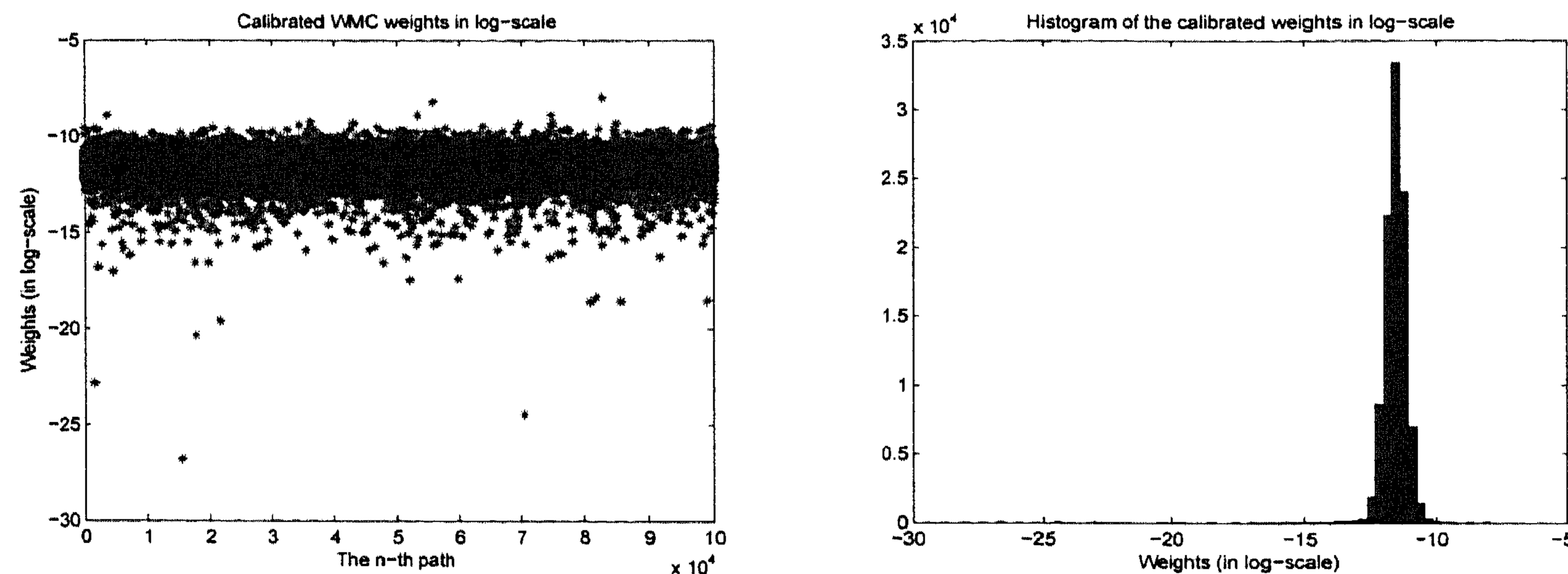
Figure 4.5: Left: a cloud plot of the 10^5 weights (in log-scale) of the WMC paths obtained after the calibration. Right: histogram of the values of the calibrated weights in log-scale.
