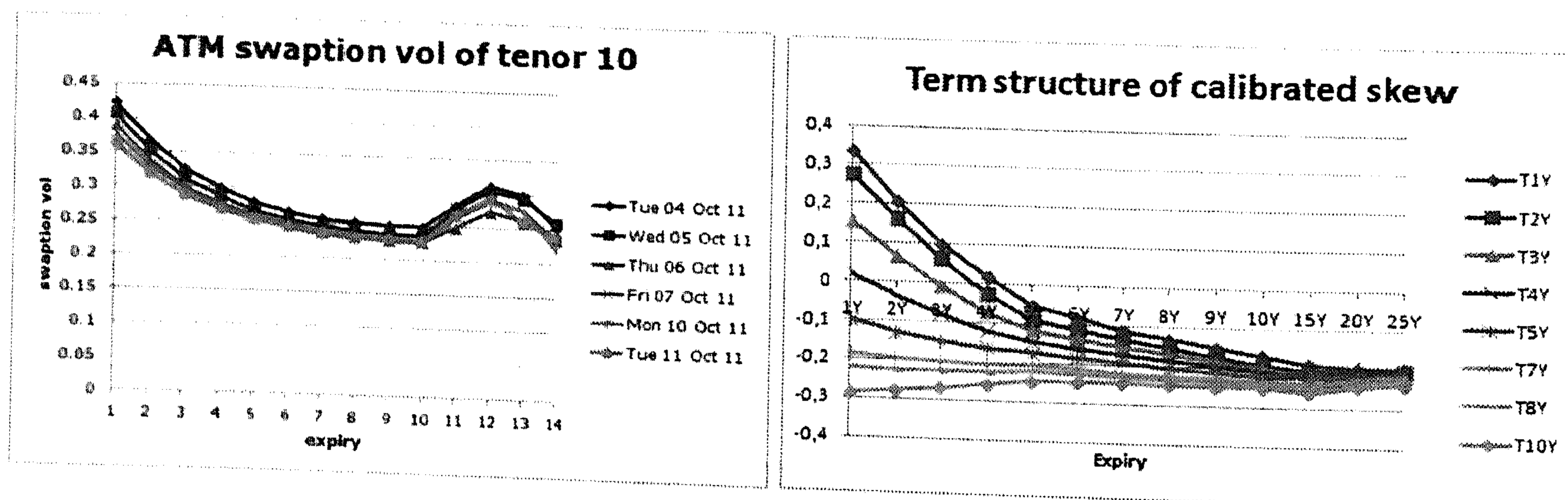
Figure 5.1: LHS: The term structure of ATM swaption volatility with tenor 10 years observed at different spot dates. RHS: The term structure of skew obtained by calibrating a constant parameter displaced Heston model to swaption prices with different combinations of expiry/tenor (T1Y stands for tenor 1 year).
