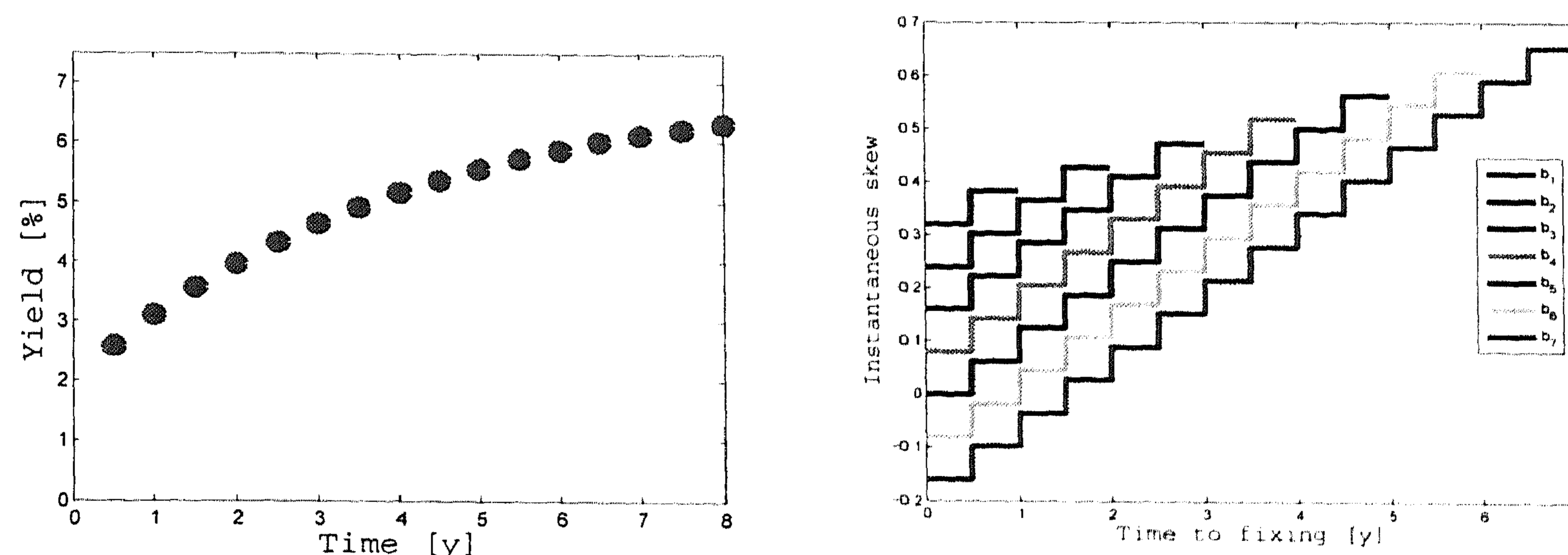
Figure 5.6: LHS: Initial yield curve for the experiment. RHS: The instantaneous LIBOR skews considered in the experiment.
