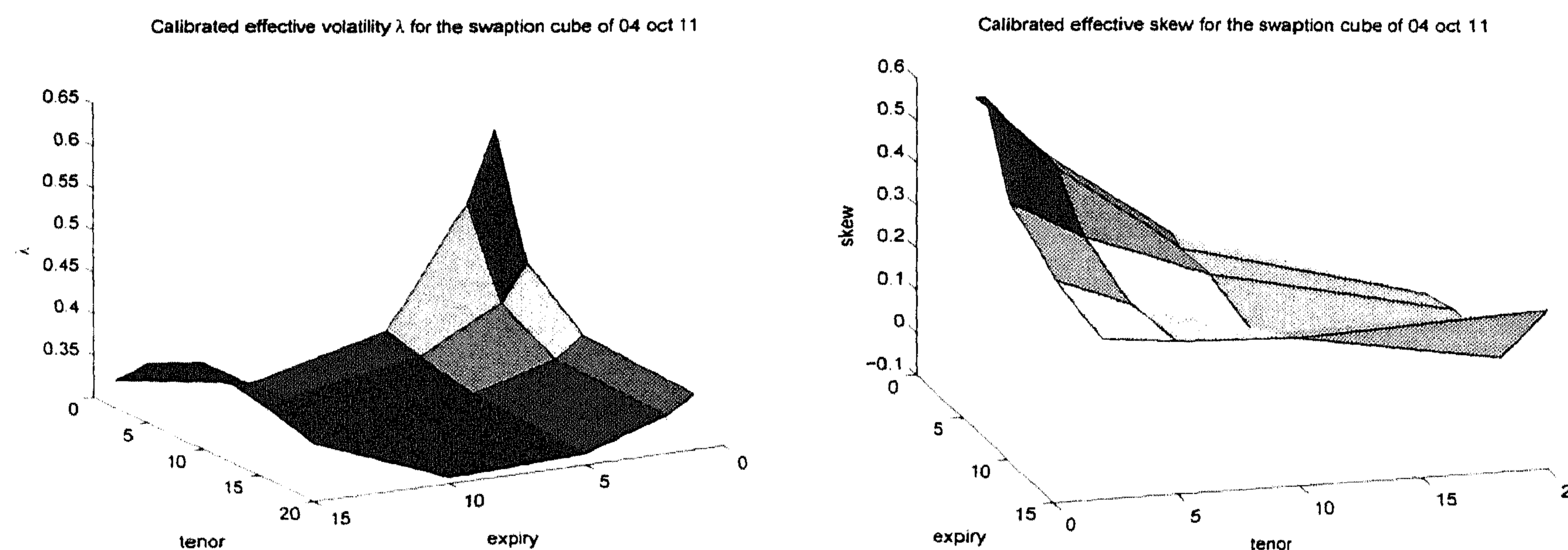
Figure 5.7: Calibrated parameters \lambda (left) and b (right) for the swaption cube of 04-oct-2011.
