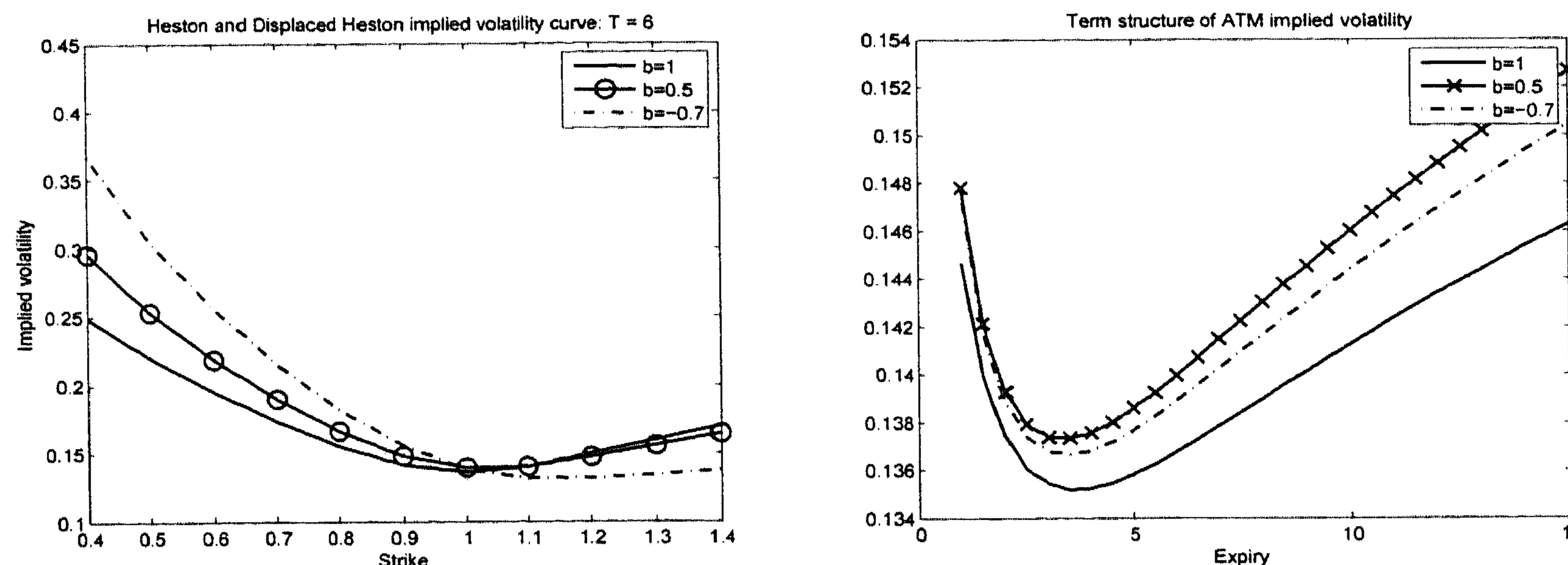
Figure 5.3: Implied volatility curve of one expiry slice and term structure of ATM implied volatility.
