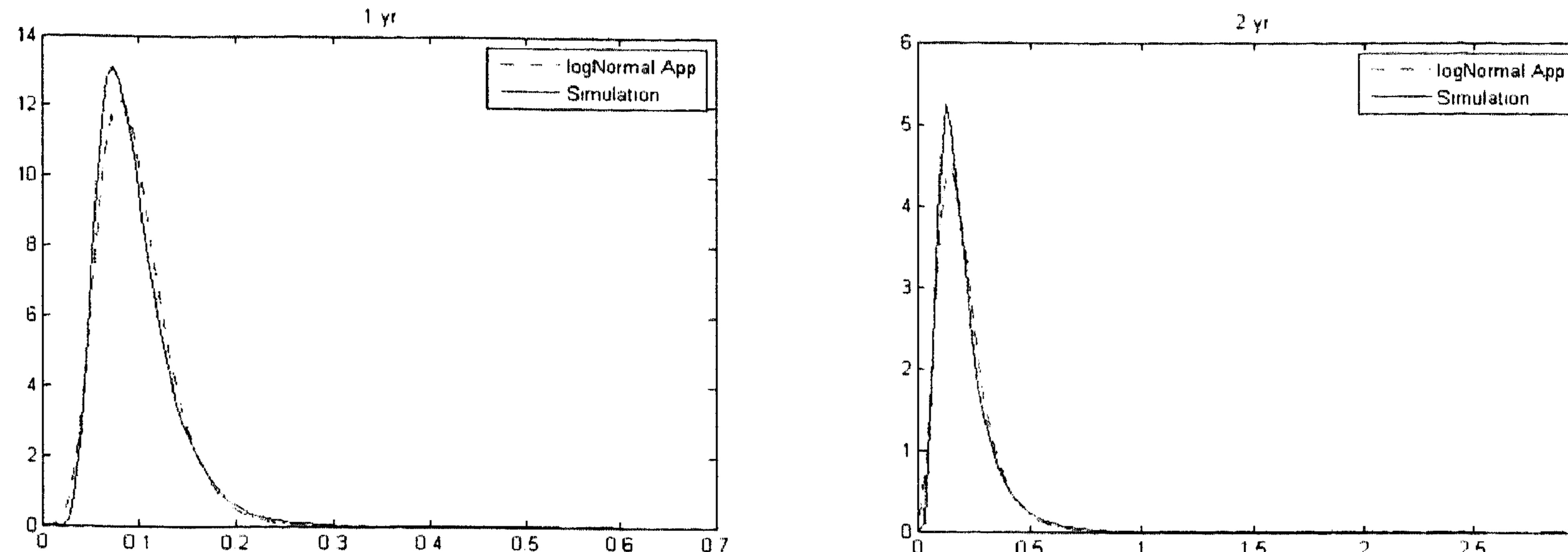
Figure 3.4: Quality of the approximation of the conditional moment-matched log-normal density compared to the true density of integrated variance, A(\Delta) . The parameters chosen are \sigma(0) = 0.4 , \alpha = 0.5 . In the LHS plot, T = 1 ; in the RHS plot T = 2 .
