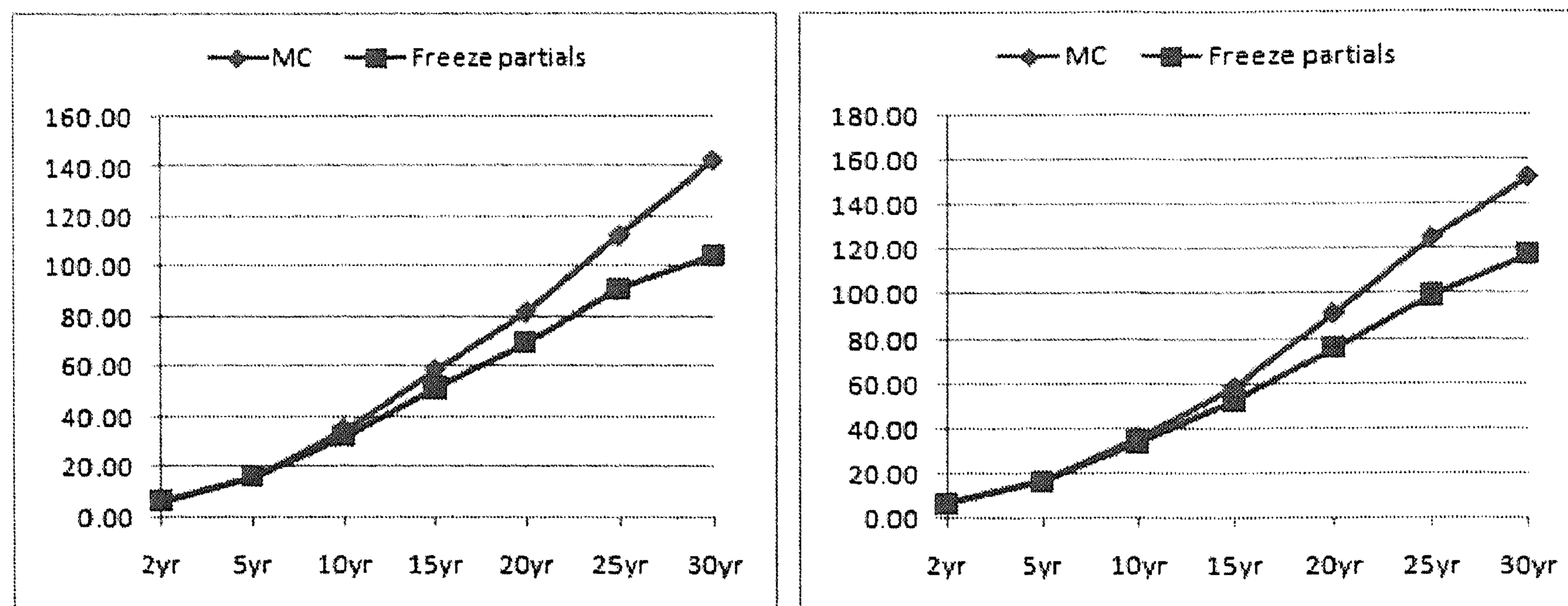
Figure 2.3: Error due to constant partial derivatives, with \beta = 1 . Left-hand side: positive correlation between swap rate and the LIBOR rate. Right-hand side: negative correlation between these two rates.
