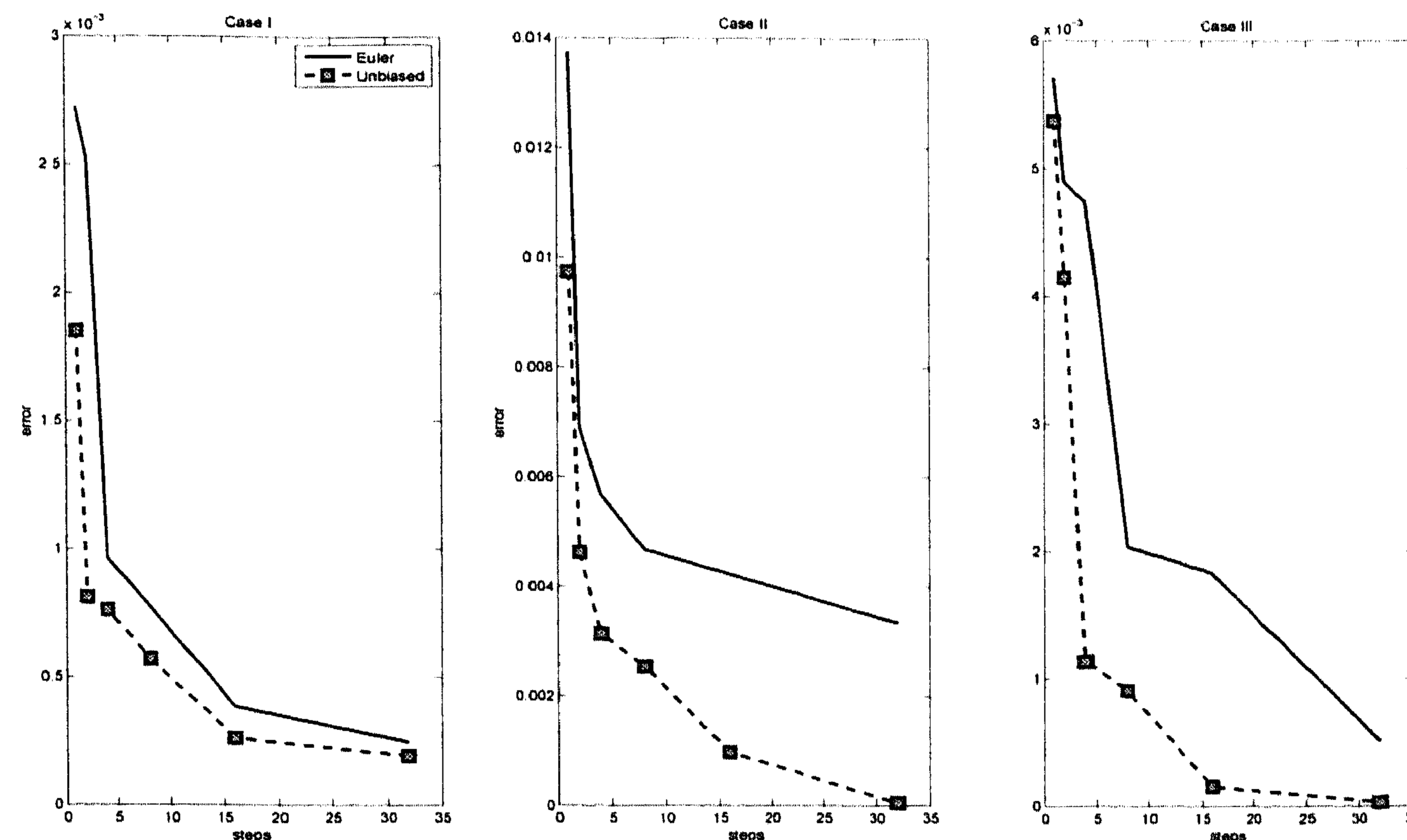
Figure 4.6: The MC error as a function of the number of time steps. Note the different scaling of the three figures.
