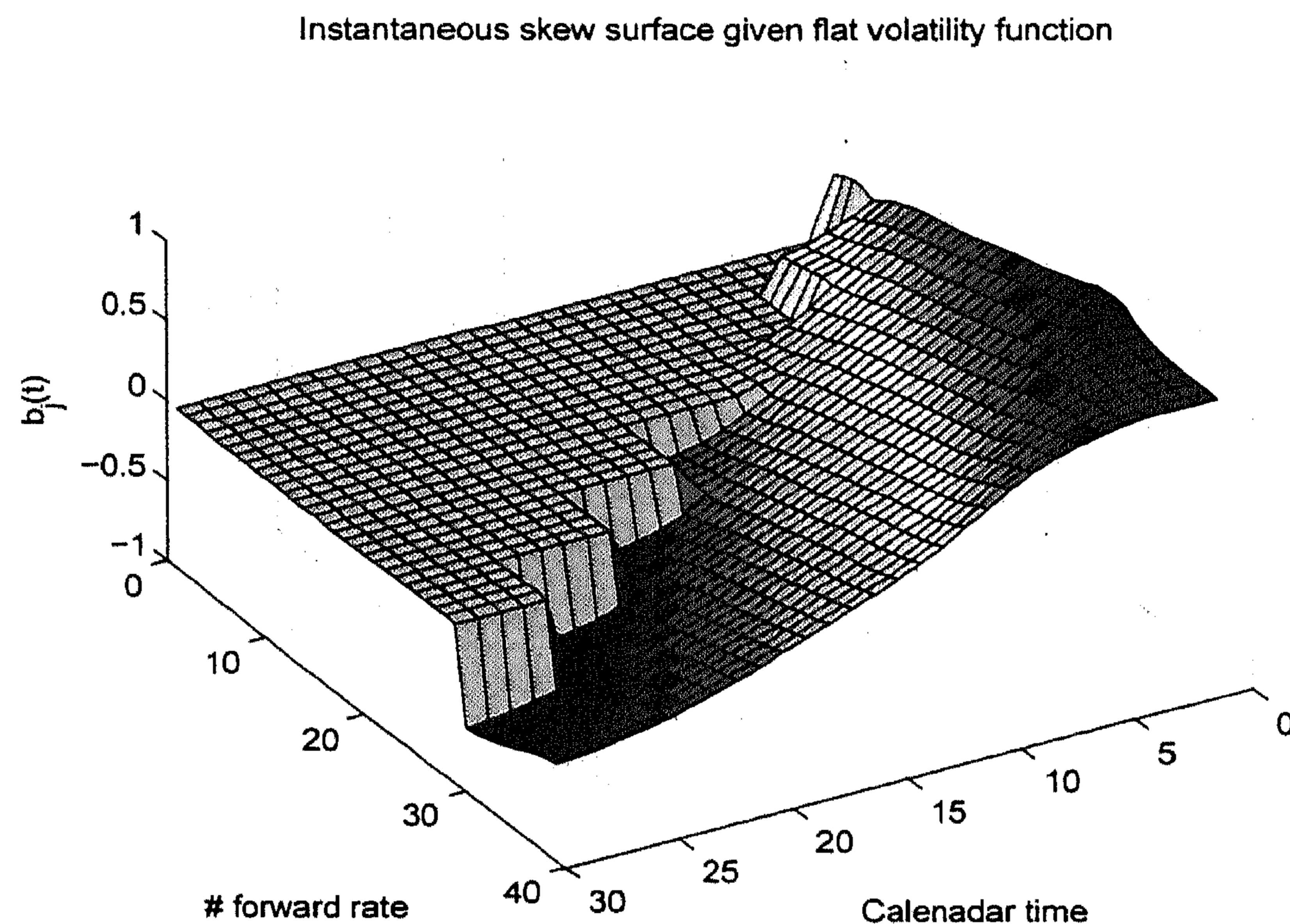
Figure 5.12: The calibrated instantaneous skew surface for the sample problem in [86].
