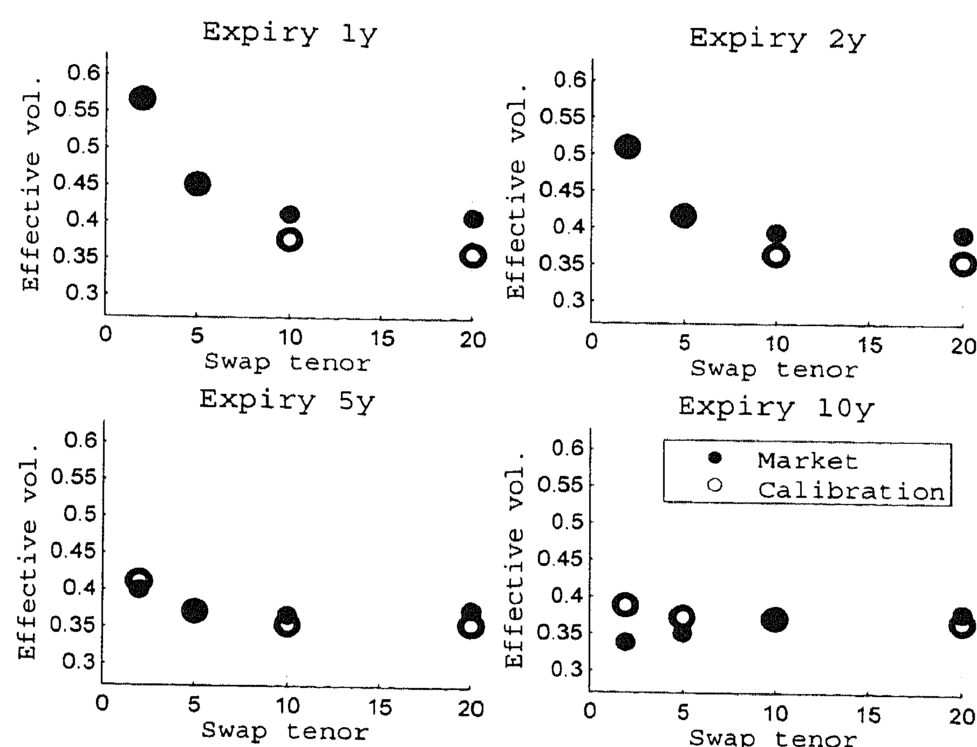
Figure 5.9: Calibrated effective volatility and the market implied effective volatility.
