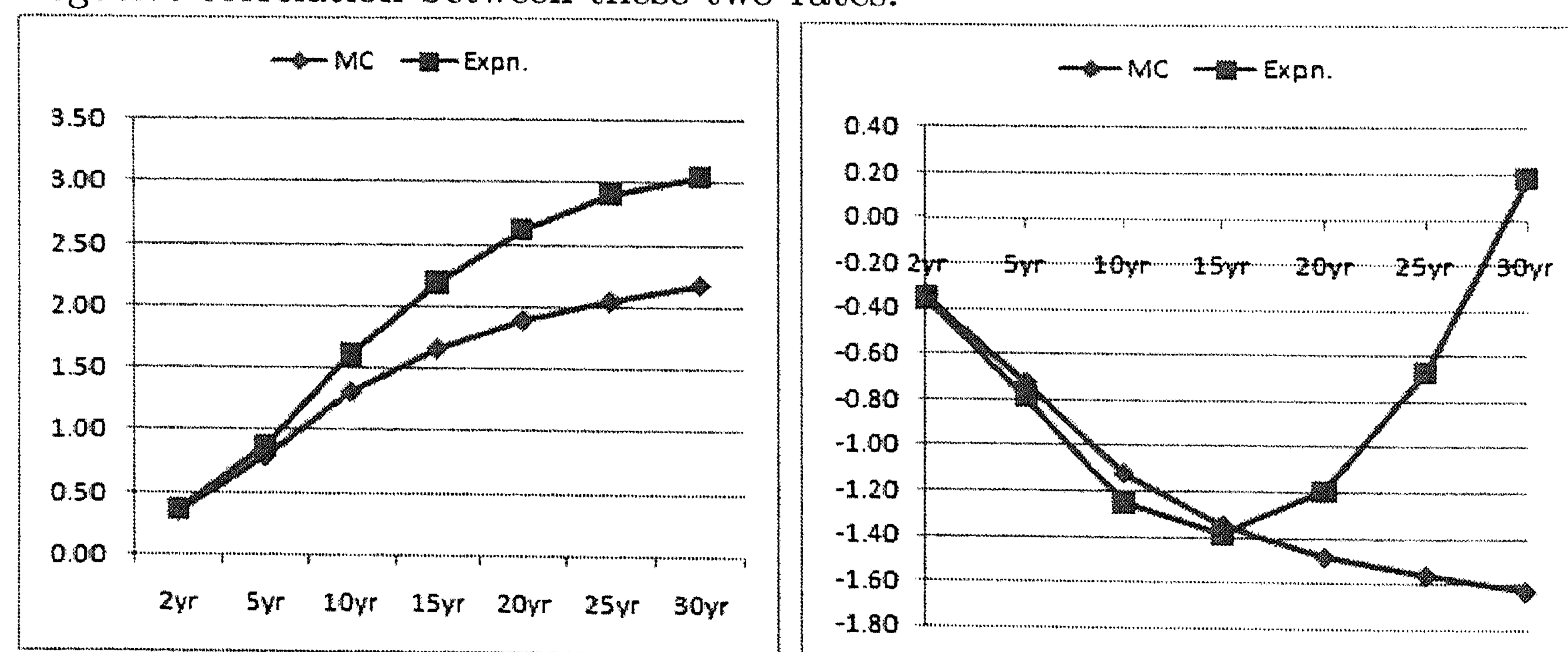
Figure 2.4: Error due to the expansion for the variance, \beta = 1 . Left-hand side: positive correlation between swap rate and the LIBOR rate; Right-hand side: negative correlation between these two rates.
